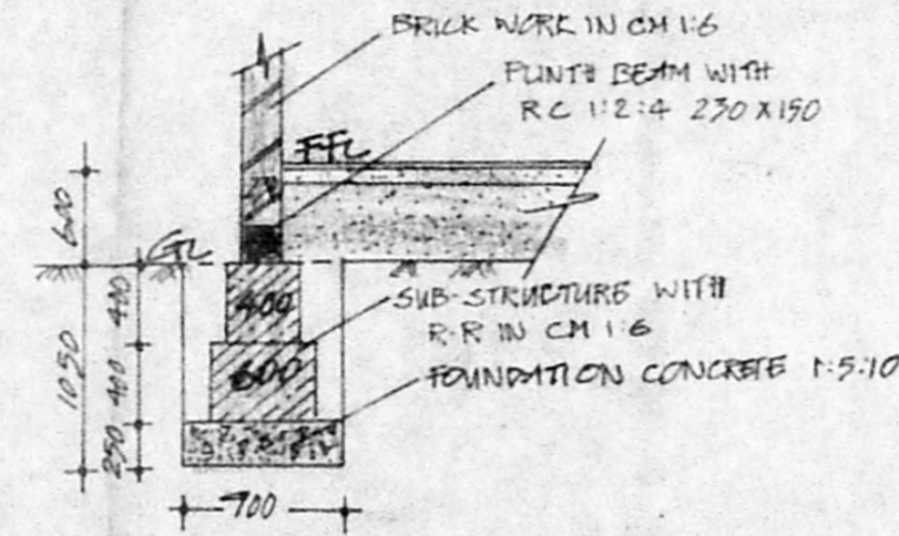
TYP-FOUNDATION (SC 1:50)
