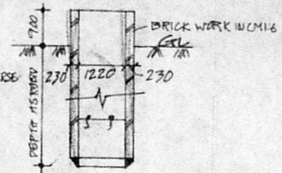
SECTION OF THE PRO WELL
